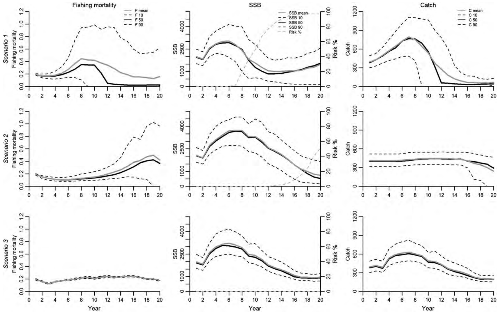
Figure 6. Summary of simulation output of three management regime scenarios for 20 years. Each panel shows the mean and 10, 50 and 90 percentiles by year. Left column: fishing mortality; centre column: spawning stock biomass (SSB) and cumulated risk of stock depletion; right column: catch. Upper row: management regime based on environmental indicators only ( Scenario 1 ). Centre row: management regime based on environmental indicators and total stock biomass indicators ( Scenario 2 ). Lower row: management regime based on estimated stock abundance and fixed harvest rate ( Scenario 3 ). Please refer to text for further definition of decision rules (Table 3) and of risk.
