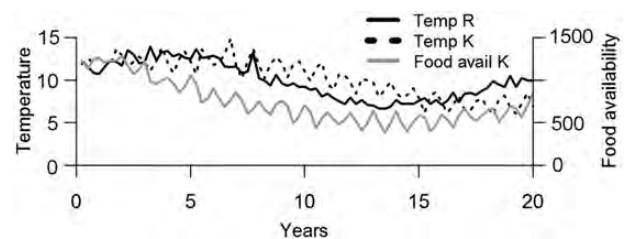
Figure 4. Time-course of environmental variables in the worked example. The variables include temperature associated with recruitment ( Temp R ), temperature ( Temp K ), and food availability associated with growth.
