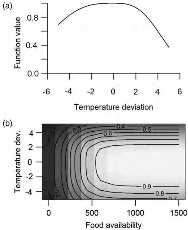
Figure 2. Examples of output from link functions. (a) An example of the asymmetric bell link function (equation 10 in text), with deviation of a temperature indicator from a normal value along the x-axis. (b) A link function made by multiplying an asymmetric bell function of temperature deviation from a normal value with a logistic function of an environment indicator, which may represent the food availability (equation 11 in the text). The function is used to model the growth rate k , relative to a standard value, in the worked example. The grey shadings and isoclines indicate the relative k -values.
