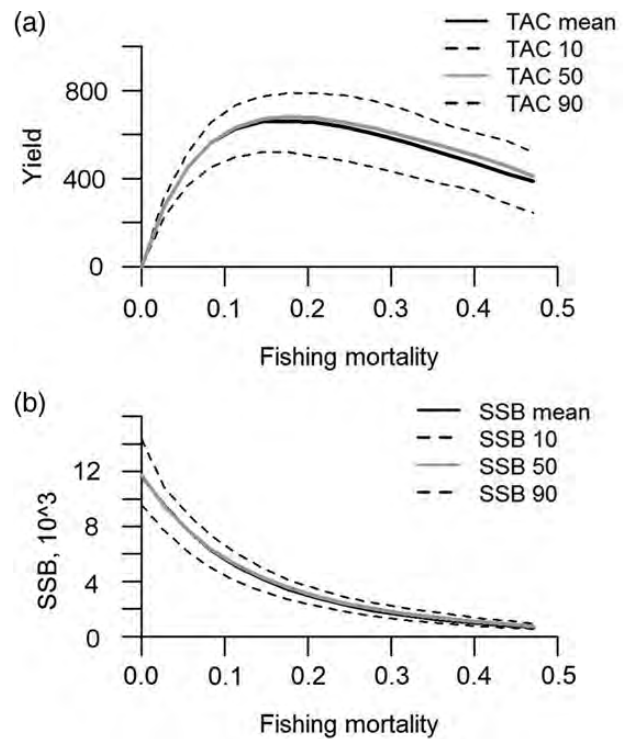
Figure 3. Characteristics of the model population in the worked example. (a) Total allowable catch (TAC), and (b) spawning stock biomass (SSB), as functions of mean fishing mortality after 20 years simulation with constant environmental influence (mean and 10, 50 and 90 percentiles).
