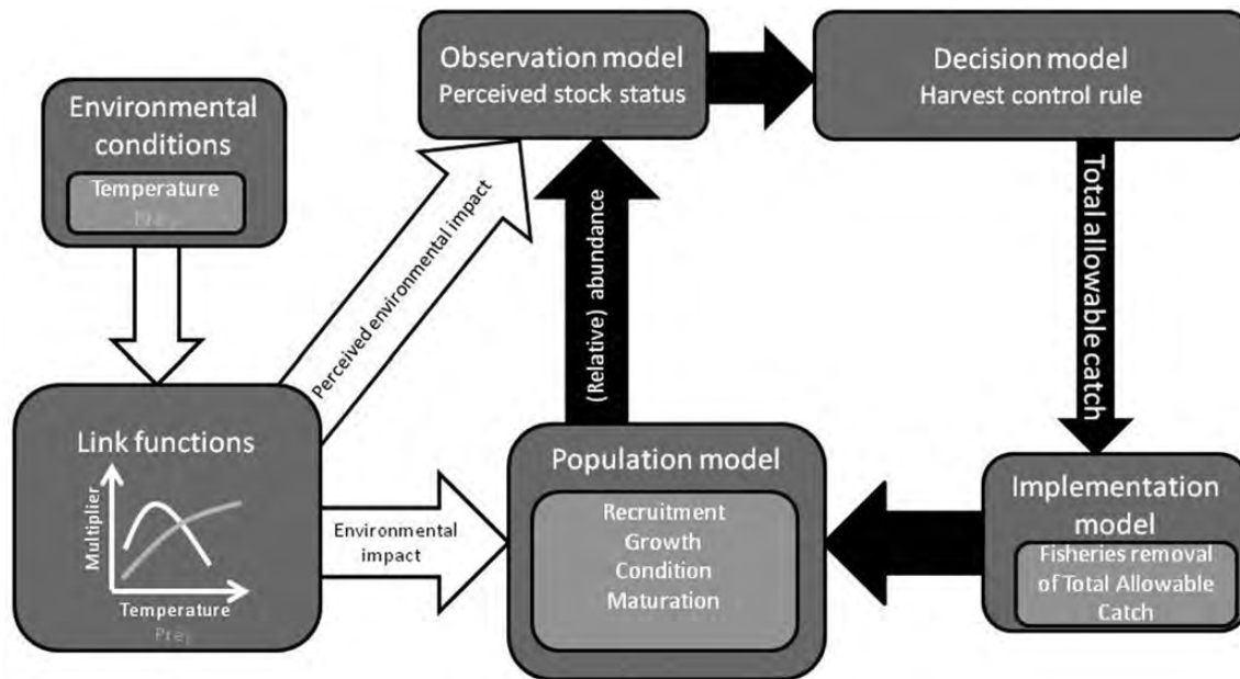
Figure 1. Schematic outline of the simulation tool kit. The boxes are processes; arrows indicate the information flow. Further details are given in the main text.
